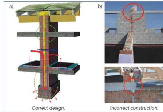
Figure 10.10. a) Example of good design for row houses. Separating walls must be structurally and acoustically separate. The cavity does not have any bridges and must be continuous from the foundations to the roof. The green circles indicate the key junctions where bridges have to be avoided. b) Incorrect workmanship. Mortar connects both leaves of the wall. (The decrease can vary from 3 dB to 12 dB, depending where and how many bridges can be found within the cavity wall).
