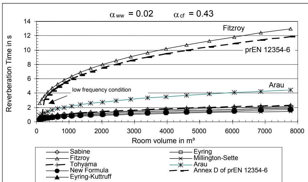
Fig. 6. Calculated reverberation time using various calculation formulae for high absorption of the floor and low absorption of other surfaces (there is an average absorption applied to the ceiling)
